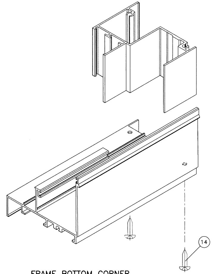
FRAME BOTTOM CORNER
